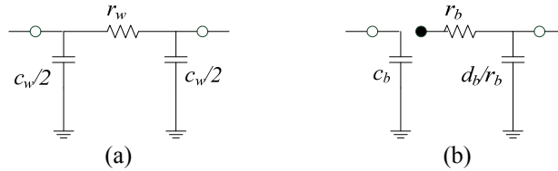
Fig. 2. (a) Wire segment model. (b) Buffer model.
